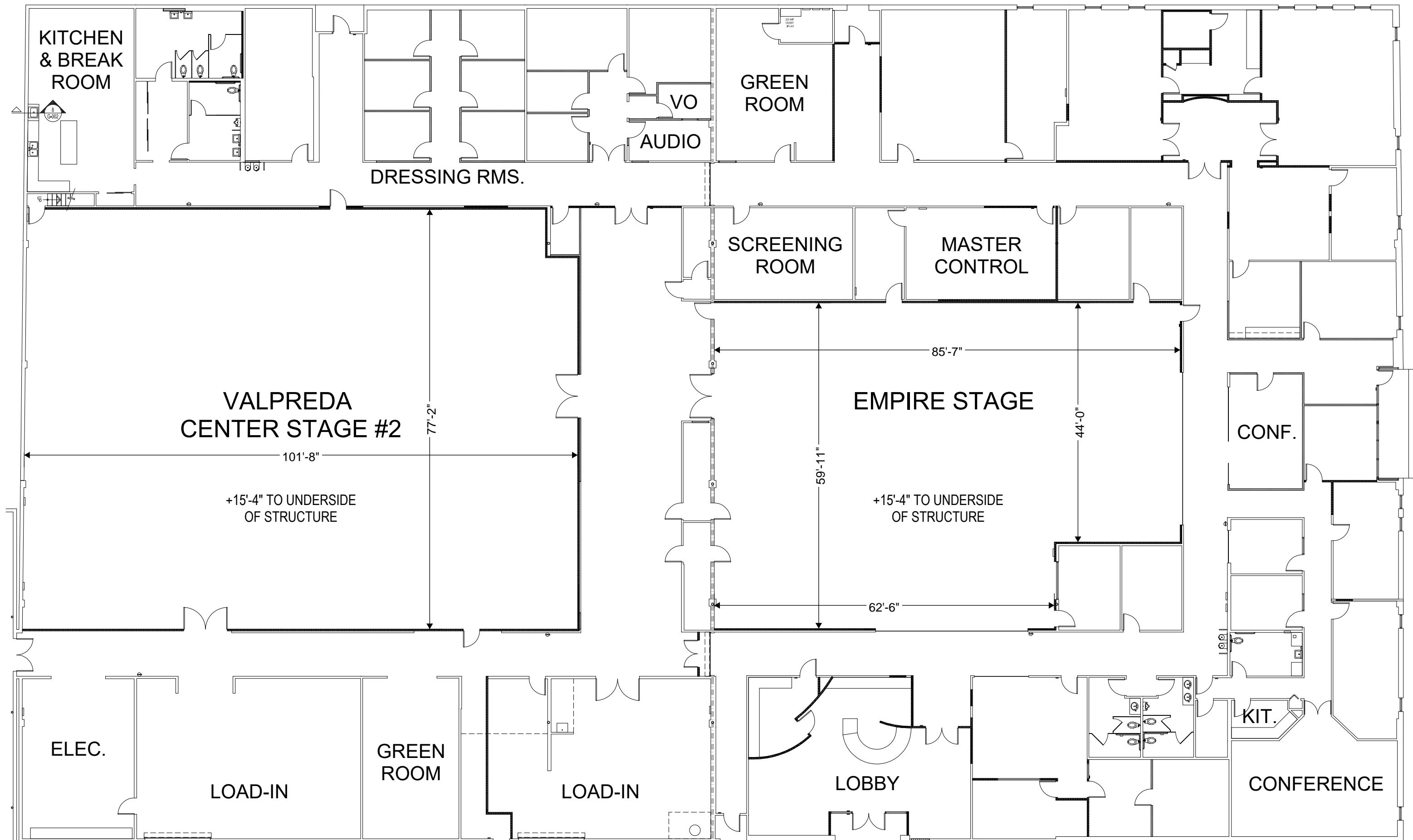
FIRST FLOOR SCALE: 1/16" = 1'-0"
